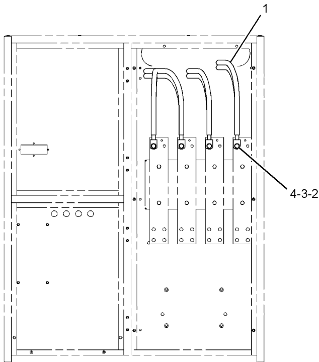
(BREAKER CONNECTION)
