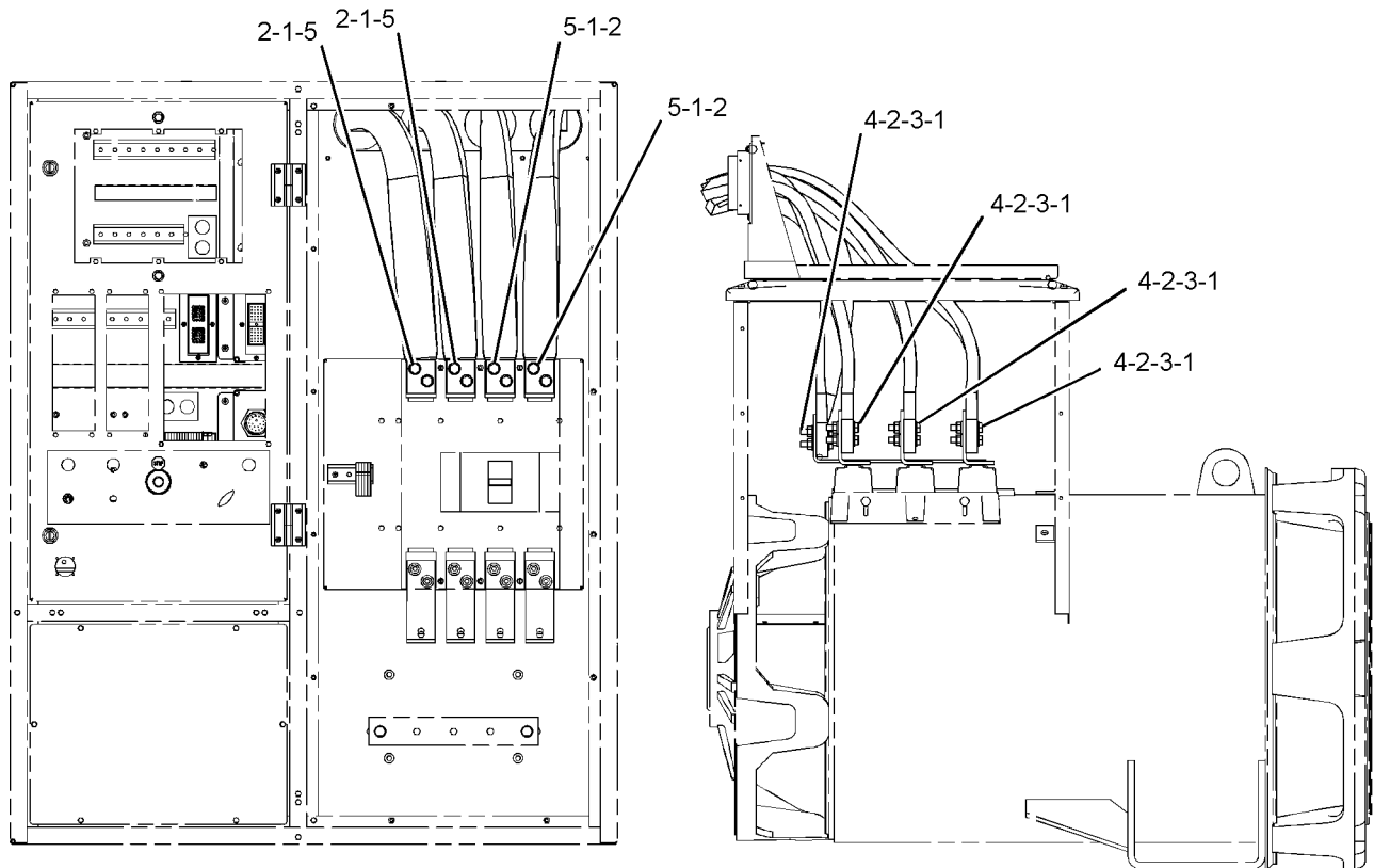
BREAKER CONNECTION
