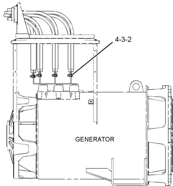
(ALTERNATOR CONNECTION)
