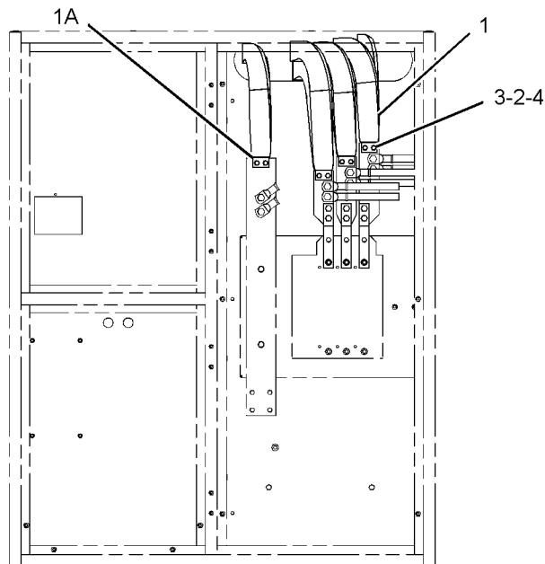
BREAKER CONNECTION
